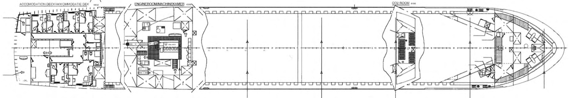
ACCOMMODATION DECK/AKKOMMODATIE DEK
